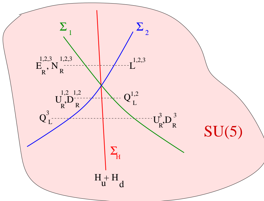
Figure 3: Sketch of the structure of the hypercharge fluxed SU(5) model.
