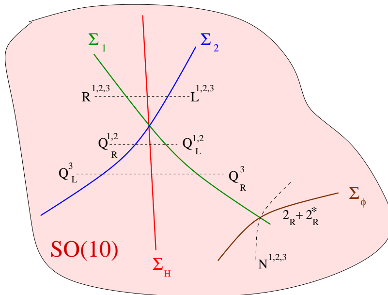
Figure 2: Sketch of the structure of the B - L fluxed SO(10) model. Dashed lines represent fermions linked by a Yukawa coupling. Yukawa couplings for all fermions are allowed.
